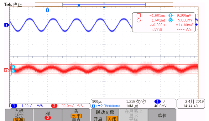
18. 纹波抑制比 (VIN=6.0V, IL=50mA, Vpp=1V, F=1KHZ)
